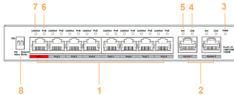
Figure 2-1 Front panel
